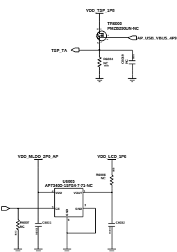
OCTA LDO(VDDR)
